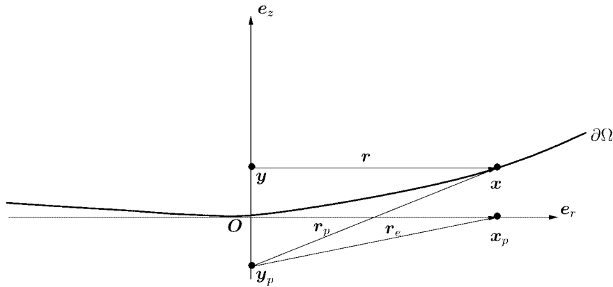
Fig. 1. Definition of the various points and displacement vectors which are utilized in the proof of Lemma 1 and Theorem 1.
