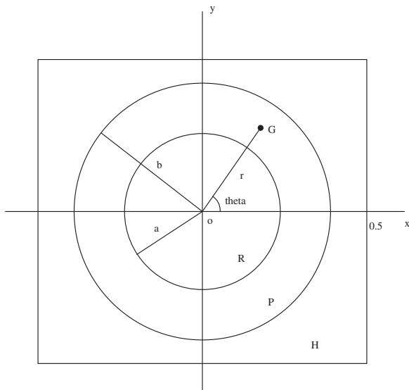
Fig. 2. The period cell: R represents the high dielectric core, P the plasmonic coating and H denotes the connected host material.
