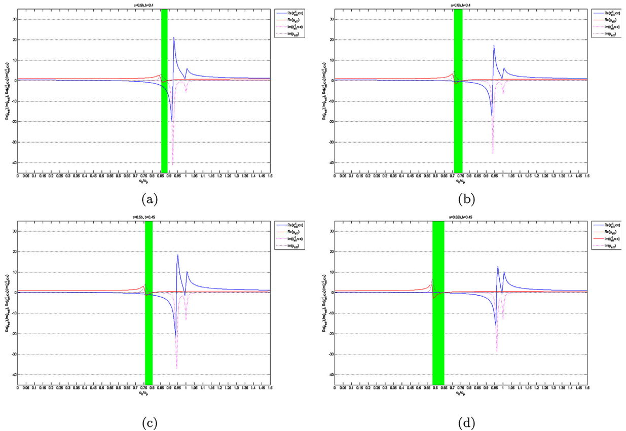
Fig. 3. Real and imaginary part of the effective permittivity and permeability associated with different choice of inner and outer radii for the coating, when \epsilon_R = 200 + i5 and \omega_c/\omega_p = 0.01 . The green strip gives the interval where the real parts of \mu_r = \mu_{eff} and \epsilon_r = \epsilon_{eff}^{-1} \hat{k} \cdot \hat{k} / |\epsilon_{eff}^{-1} \hat{k} \cdot \hat{k}|^2 are both negative. (a) For a = 0.5b , b = 0.4 ; (b) for a = 0.6b , b = 0.4 ; (c) for a = 0.5b , b = 0.45 ; (d) for a = 0.65b , b = 0.45 . (For interpretation of the references to color in this figure legend, the reader is referred to the web version of this article.)
