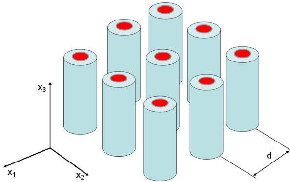
Fig. 1. Periodic array of coated dielectric rods with period d .
