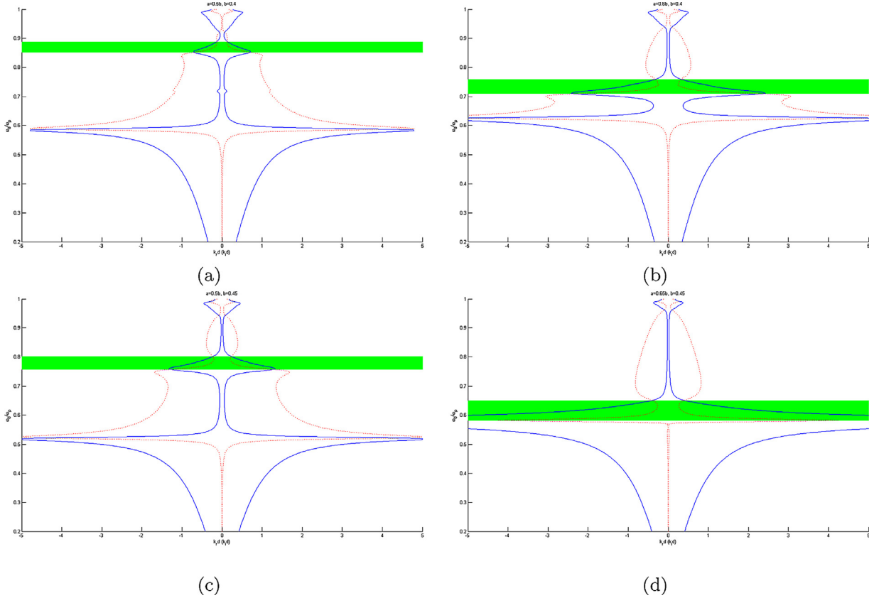
Fig. 4. Dispersion curves associated with different choice of inner and outer radii for the coating, when \epsilon_R = 200 + i5 and \omega_c/\omega_p = 0.01 . The dashed line corresponds to the imaginary part dk_i , the solid line corresponds to the real part dk_r . The green stip gives the interval where Re(\mu_{eff}) and Re(\epsilon_{eff}^{-1}\hat{k} \cdot \hat{k}) are both negative. (a) is for a = 0.5b, b = 0.4 ; (b) for a = 0.6b, b = 0.4 ; (c) for a = 0.5b, b = 0.45 ; (d) for a = 0.65b, b = 0.45 . (For interpretation of the references to color in this figure legend, the reader is referred to the web version of this article.)
