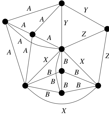
FIGURE 3. Theorem 6.4 fails for the cycle matroid of this graph G .
