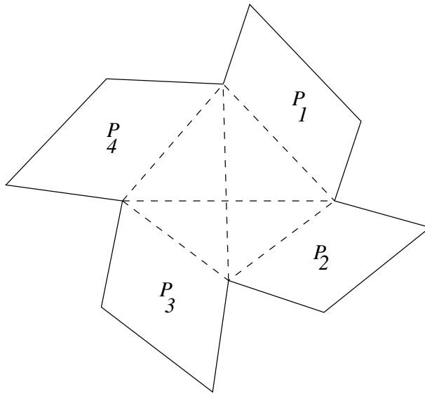
FIGURE 2. A representation of a rank-7 swirl-like flower.
