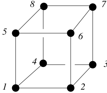
FIGURE 4. Theorem 8.1 fails for this matroid, R_8 .
