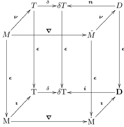
FIGURE 1. QS calculus commutative diagram. Here \delta has been used to denote the variation \delta T = T_t - T_0 of the operator T , and \nabla is the single point split operator [13, 9].
