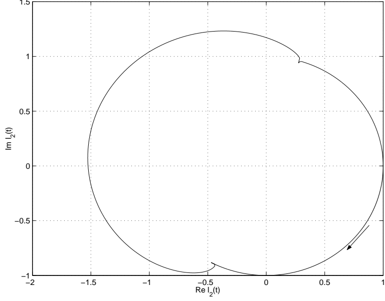
Figure 4: The set \{l_2(t) : 0 < t < 1\} , for \beta = \frac{1}{4}\pi , \eta_2^+/\eta_1^+ = 0.001 , \eta_1^-/\eta_1^+ = 10 , \eta_2^-/\eta_1^+ = 2 .
