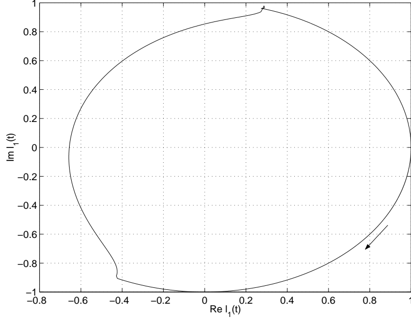
Figure 3: The set \{l_1(t) : 0 < t < 1\} , for \beta = \frac{1}{4}\pi , \eta_2^+/\eta_1^+ = 0.001 , \eta_1^-/\eta_1^+ = 10 , \eta_2^-/\eta_1^+ = 2 .
