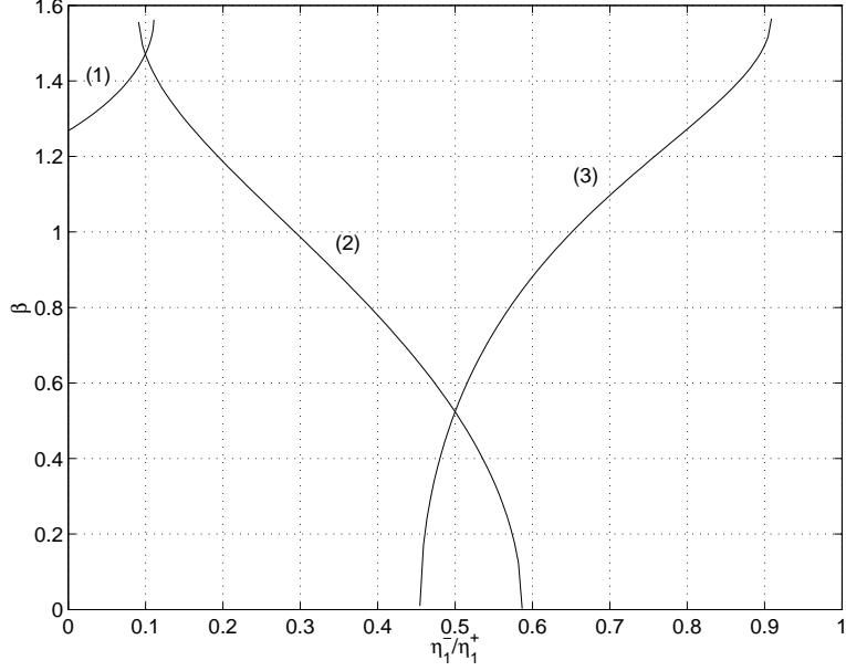
Figure 5: Some cases when \rho = -1 . The angle of incident \beta vs \eta_1^-/\eta_1^+ for (1) \eta_2^+/\eta_1^+ = 0.01 , \eta_2^-/\eta_1^+ = 10 ; (2) \eta_2^+/\eta_1^+ = 2 , \eta_2^-/\eta_1^+ = 10 ; (3) \eta_2^+/\eta_1^+ = 2 , \eta_2^-/\eta_1^+ = 0.1 .
