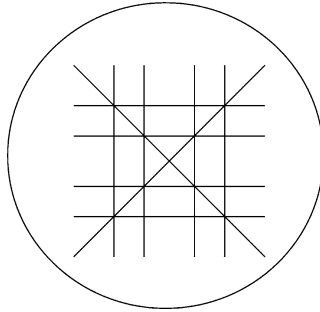
Fig. 1. The coned fiber arrangement, for \ell = 4 .
