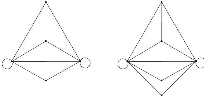
Fig. 2. Extensions of Theorem 5.6.
