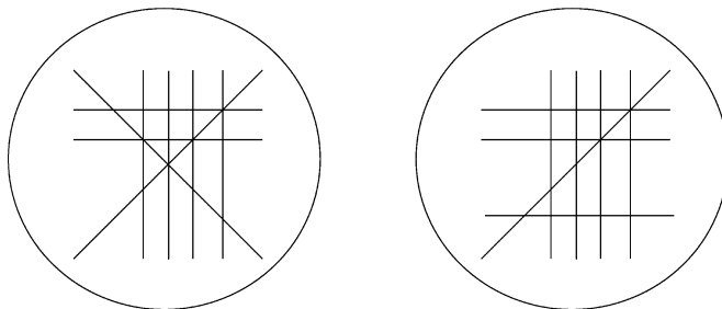
Fig. 4. Two non- K(\pi, 1) arrangements.
