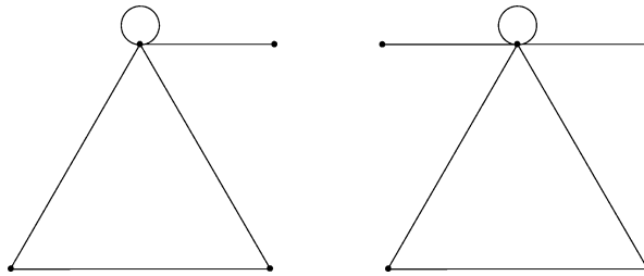
Fig. 3. Graphs of K(\pi, 1) extensions of a non-Fano arrangement.
