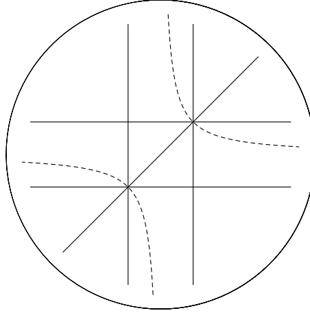
Fig. 1. The braid arrangement with \text{crit}(\Phi_{1,1,-2})
