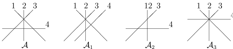
FIGURE 1. A line arrangement and three degenerations
