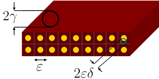
Figure 3: Long-range bonds (horizon \gamma ) and short-range bonds (horizon \epsilon\delta ).
