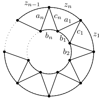
FIGURE 13. A labelled quartic ladder.
