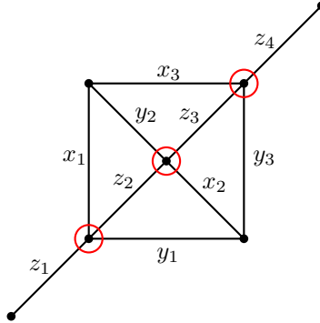
FIGURE 2. An augmented 4-wheel.
