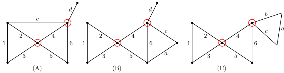
FIGURE 13. In each structure, we view the labels on 2 and 3 as being interchangeable. The elements in each part are distinct except that a may equal 1 in (B) and (C).
