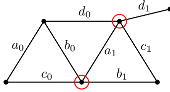
FIGURE 18. The elements in this structure are all distinct, and we view the labels on a_1 and b_1 as being interchangeable. Furthermore, d_1 \in Y , and either d_0 \in X or M' \setminus c_0, c_1, d_0 has an N -minor.
