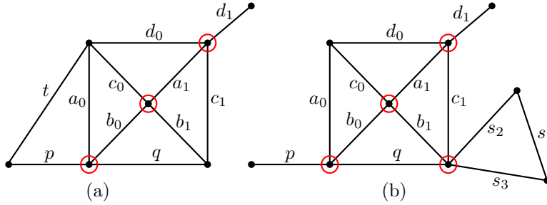
FIGURE 17. The elements in both structures are all distinct, and we view the labels on a_1 and b_1 as being interchangeable.
