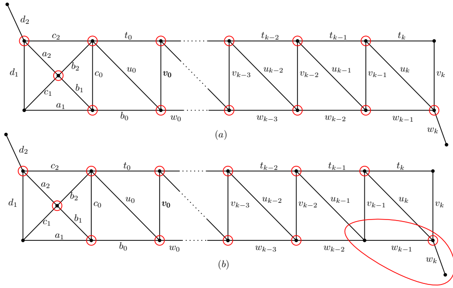
FIGURE 4. In both (a) and (b), the elements shown are distinct, except that d_2 may be w_k . Furthermore, in (a), k \geq 0 ; and in (b), k \geq 1 and \{w_{k-2}, u_{k-1}, v_{k-1}, u_k, v_k\} is a cocircuit.
