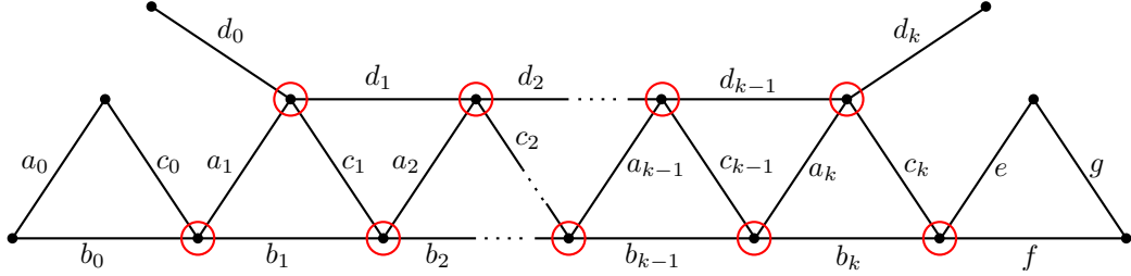
FIGURE 15. All of the elements are distinct except a_0 may be g , or T_0 may be \{e, f, g\} .
