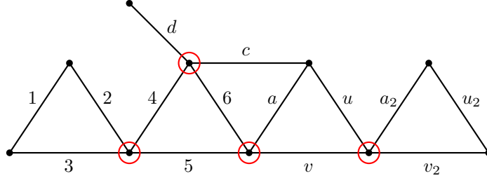
FIGURE 27. All of the elements are distinct except that u_2 may be the same as 1, or \{1, 2, 3\} may be \{a_2, u_2, v_2\} .
