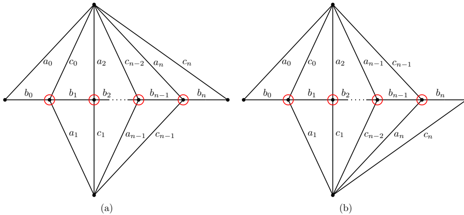
FIGURE 10. Right-maximal rotor chain configurations. In the case that n is even, the rotor chain is depicted on the left. If n is odd, then the rotor chain has the form on the right.
