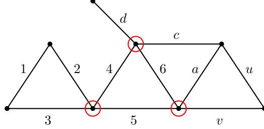
FIGURE 26. All of the elements are distinct except that u may be 1.
