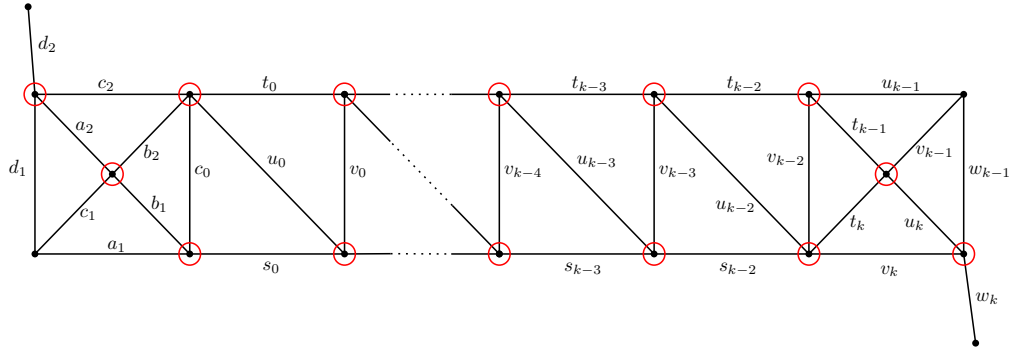
FIGURE 5. In this configuration, k \geq 2 and the elements are all distinct except that d_2 may be w_k .
