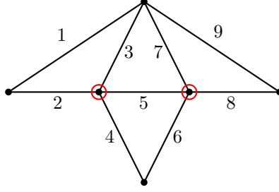
FIGURE 9. A quasi rotor, where \{2, 3, 4, 5\} and \{5, 6, 7, 8\} are cocircuits.
