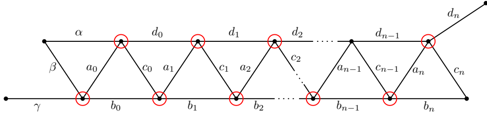
FIGURE 11. n \geq 1 and M has either \{d_{n-2}, a_{n-1}, c_{n-1}, d_{n-1}\} or \{d_{n-2}, a_{n-1}, c_{n-1}, a_n, c_n\} as a cocircuit, where d_{-1} = \alpha if n = 1 .
