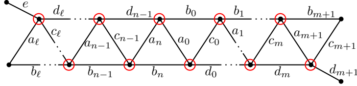
FIGURE 20. The elements depicted are all distinct, \ell \leq n , where we let d_n = b_0 , and m \geq 0 . Furthermore, m \leq \ell - 2 .
