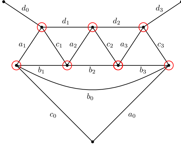
FIGURE 14. All of the elements are distinct and \{b_0, b_1, b_2, b_3\} is a circuit of M .
