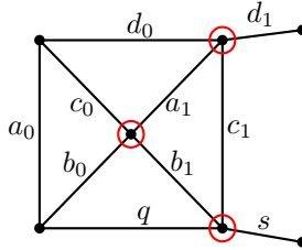
FIGURE 22. We view the labels a_1 and b_1 as being interchangeable. The elements shown are distinct.
