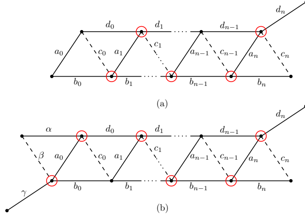
FIGURE 6. In (a) and (b), n \geq 2 and the elements shown are distinct, with the exception that d_n may be the same as \gamma in (b). Either \{d_{n-2}, a_{n-1}, c_{n-1}, d_{n-1}\} or \{d_{n-2}, a_{n-1}, c_{n-1}, a_n, c_n\} is a cocircuit in (a) and (b). Either \{b_0, c_0, a_1, b_1\} or \{\beta, a_0, c_0, a_1, b_1\} is also a cocircuit in (b).
