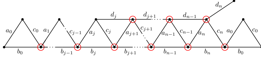
FIGURE 16. All of the elements are distinct except those with the same label.
