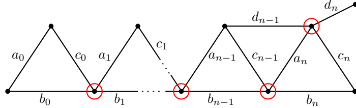
FIGURE 21. We view the labels a_n and b_n as being interchangeable. These elements are all distinct with the possible exception that (a_0, b_0) may be (c_n, d_n) in the case that n > 1 . Furthermore, if n > 1 , then d_{n-1} \notin Y .
