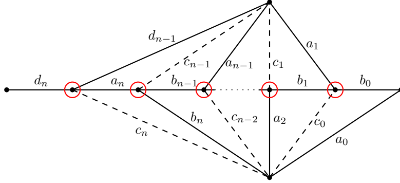
FIGURE 23. These elements are all distinct.
