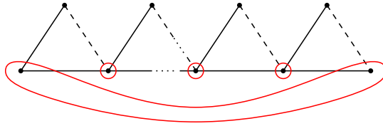
FIGURE 7. A bowtie ring. All elements are distinct. The ring contains at least three triangles.
