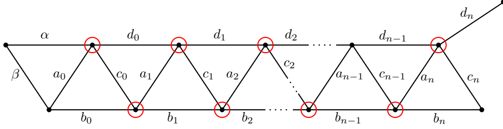
FIGURE 12. Either \{d_{n-2}, a_{n-1}, c_{n-1}, d_{n-1}\} or \{d_{n-2}, a_{n-1}, c_{n-1}, a_n, c_n\} is a cocircuit, where d_{-1} = \alpha .
