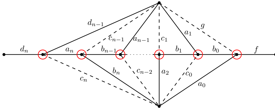
FIGURE 24. These elements are all distinct except that f may be d_n . No set in \{\{f, g\}, \{c_n, d_n\}, \{d_{n-1}, d_n\}\} is contained in a triangle. Deleting the dashed elements preserves an N -minor.
