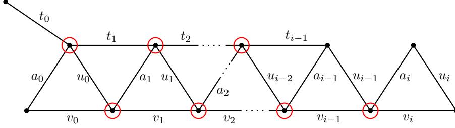
FIGURE 28. All of the elements shown are distinct.
