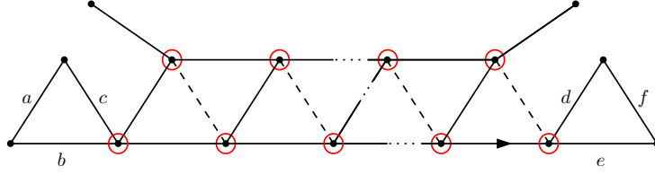
FIGURE 8. All of the elements are distinct except that a may be f , or \{a, b, c\} may be \{d, e, f\} . There are at least three dashed elements.
