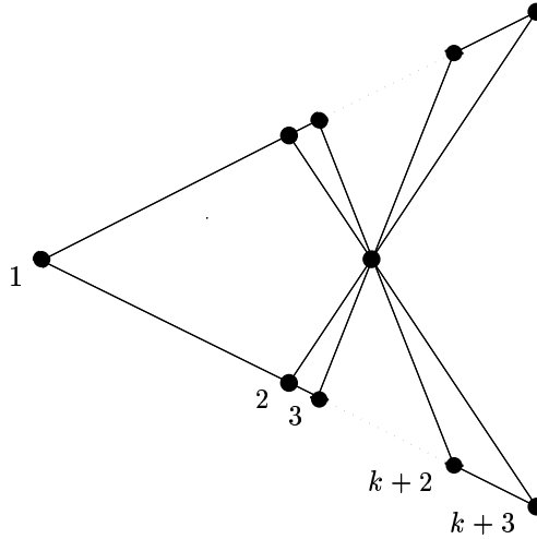
FIGURE 1. The matroid T_3^k .
