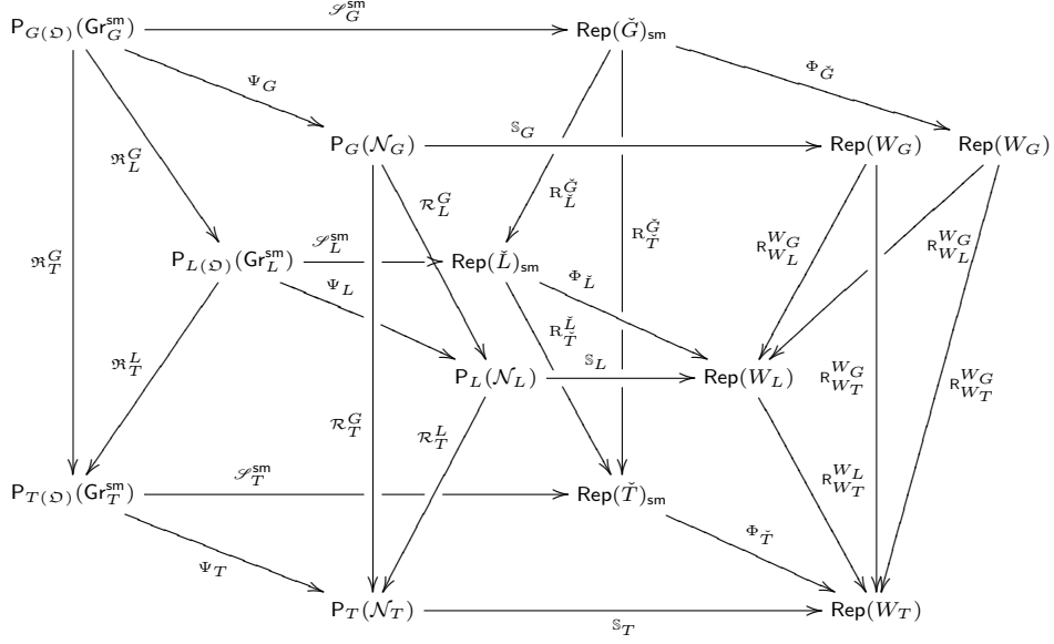
FIGURE 3.1. Diagram for the proof of Theorem 3.3. (Here, to save space, we abbreviate \mathrm{P} = \mathrm{Perv} .)
