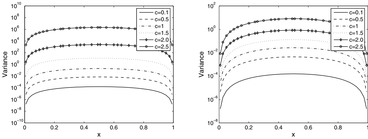
FIGURE 3. Variance of the solution for different values of c . Left: ordinary product; right: Wick product.
